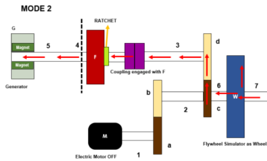
FIGURE 5. Workflow diagram of FRCS Mode 2
