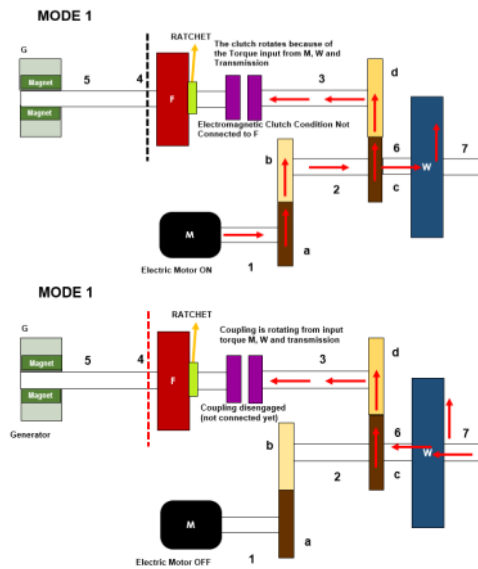
FIGURE 4. Workflow diagram of FRCS Mode 1
