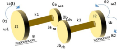
FIGURE 7. 4DOF Dynamic Modeling
