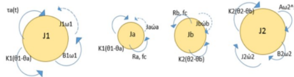
FIGURE 7. 4DOF Dynamic Modeling
