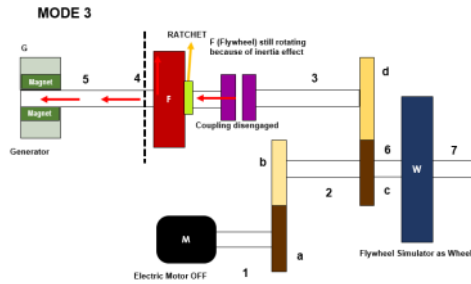
FIGURE 6. Workflow diagram of FRCS Mode 3
