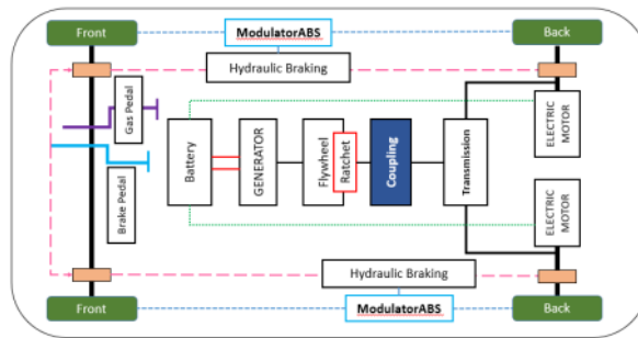
FIGURE 1. Ratchet Flywheel Regenerative System concept
