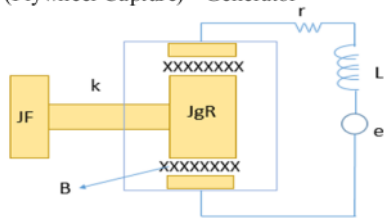
FIGURE 9. 3 DOF Dynamic Modeling
