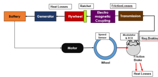
FIGURE 2. Illustration of simple FRCS concept
