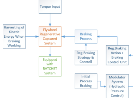
FIGURE 11. The diagram of FRCS topology
