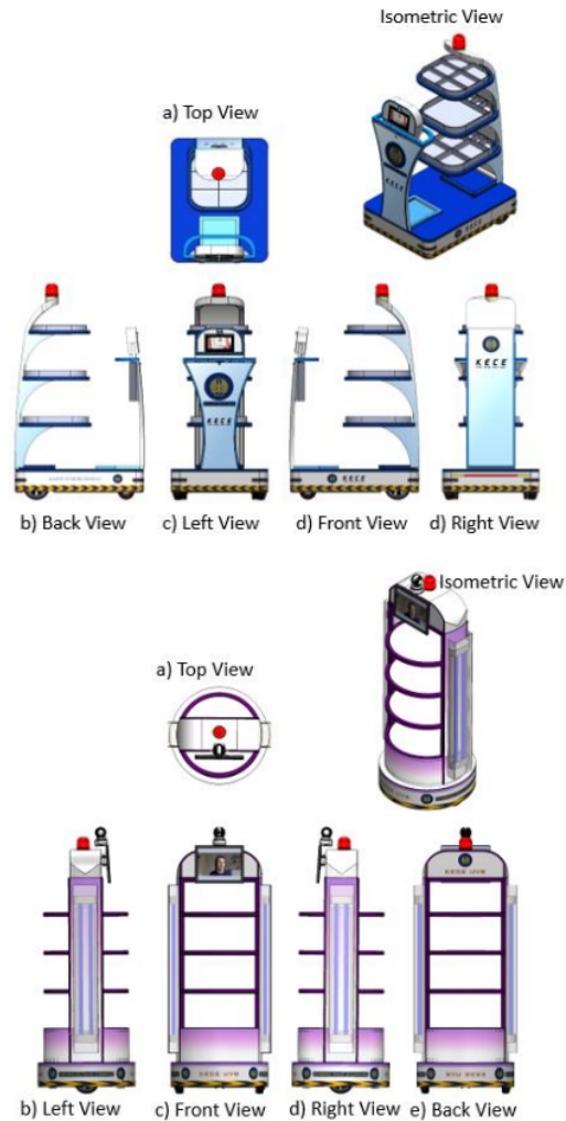
Figure 3. design of paramedic assistant robot 1.0
