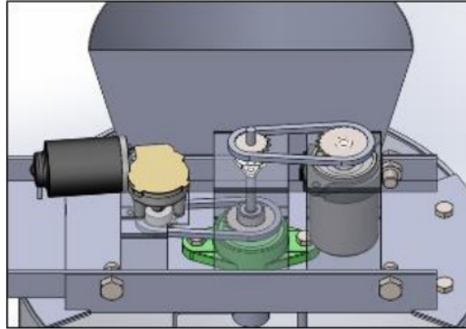
Figure 11. Redesign of Transmission
