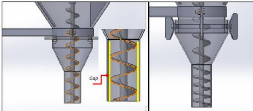
Figure 9. Redesign of Hooper
