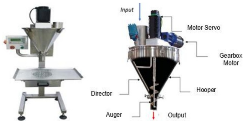
Figure 4. Fillmach S01P
