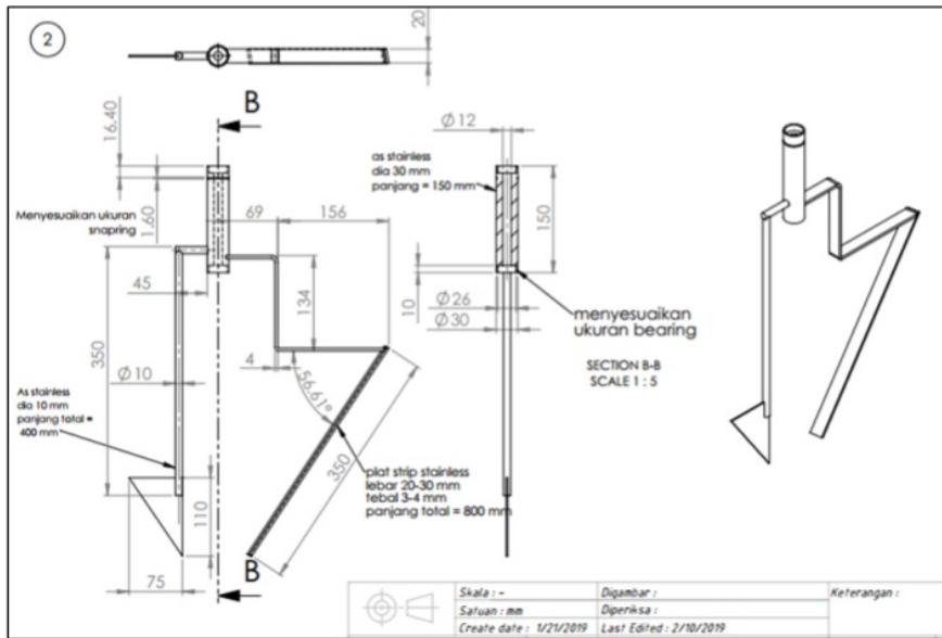
Figure 10. Redesign of Agitator
