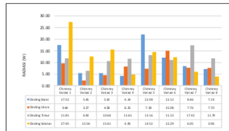
FIGURE 16. Radiation Heat Transfer Diagram In drying chamber
