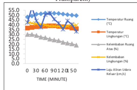
FIGURE 8. Graph Measurement Results On Variation Vertical Chimney 1.5 m (Southern and Northern Wall Transparent)
