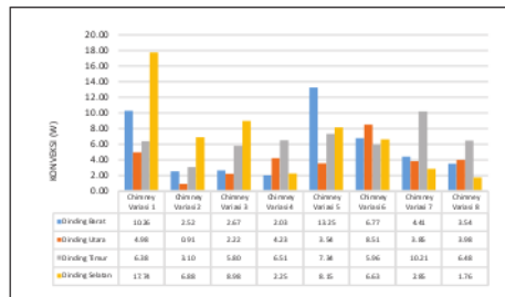
FIGURE 15. Convection Heat Transfer Diagram In Drying chamber
