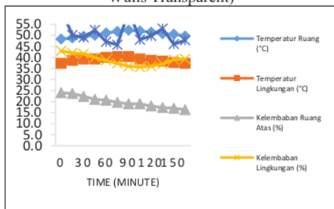
FIGURE 7. Graph Measurement Results At 1.5 m inclined Chimney Variation 45 ° (Eastern and Western Walls Transparent)
