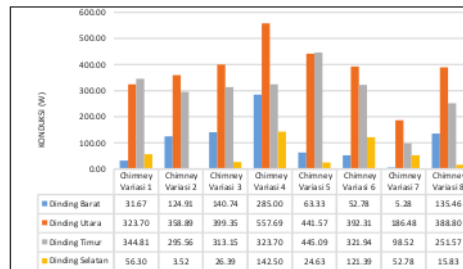
FIGURE 14. Conduction Heat Transfer Diagram On Wall Space
