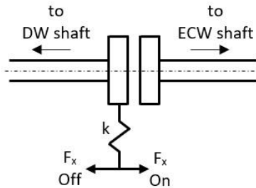
Figure 4: The centrifugal clutch
