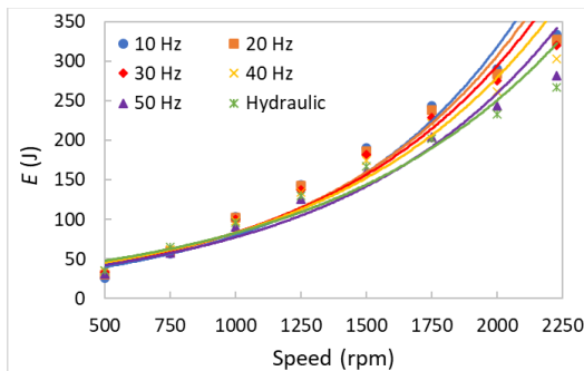
Figure 12: Energy stored from regenerative braking
