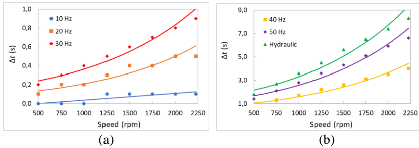
Figure 8: The difference between the stopping time to stop the wheels and the braking time to stop the vehicle: (a) lower frequency of ABS, (b) higher frequency of ABS and hydraulic
