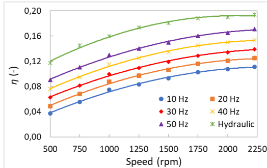
Figure 11: Regenerative braking performance
