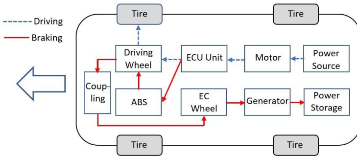
Figure 3: The vehicle configuration
