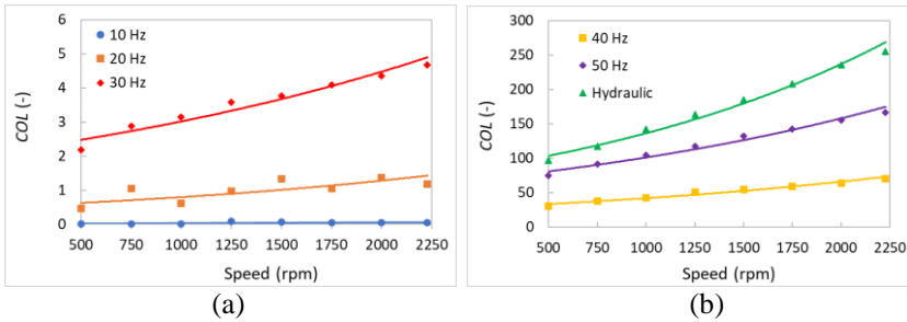
Figure 13: Coefficient of losses (COL); (a) lower frequency of ABS, (b) higher frequency of ABS and hydraulic
