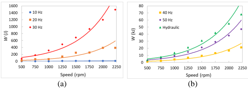
Figure 10: The friction work between the tires and the road to stop the vehicle; (a) lower frequency of ABS, (b) higher frequency of ABS and hydraulic
