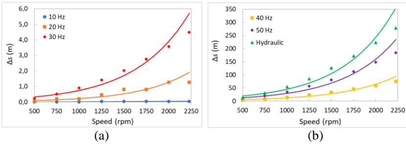
Figure 9: Distance addition stopping the vehicle: (a) lower frequency of ABS, (b) higher frequency of ABS and hydraulic
