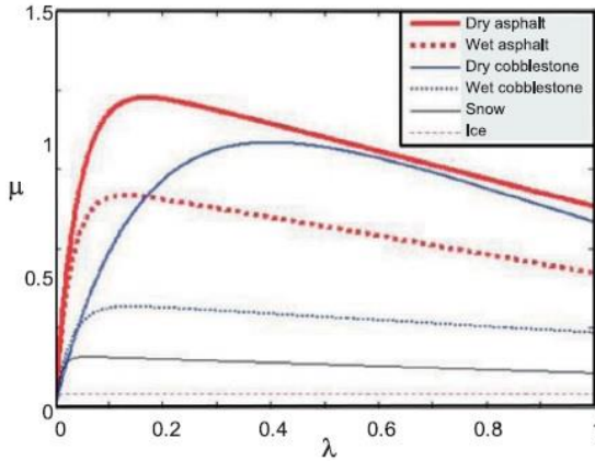
Figure 6: The friction coefficient of slip ratio function for various road conditions [25]
