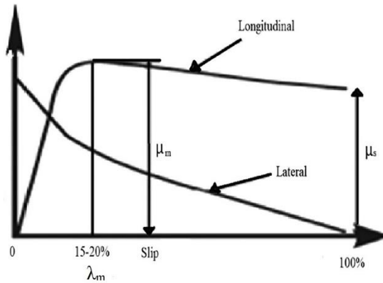
Figure 7: ABS working area at maximum friction coefficient ( \mu_m ) and maximum slip ratio ( \lambda_m ) [5]
