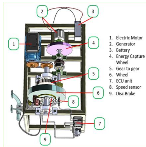
Figure 1: The vehicle components
