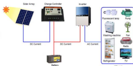
Gambar 1. Sistem model solar cell
