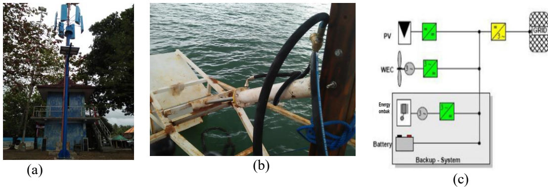
Fig. 4. Research instrument a) Solar PV-wind turbine system, b) Wave energy conversion system, (c) Hybrid electrical model
