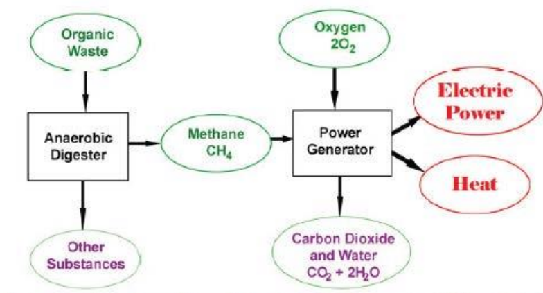
Figure 3. Model of biogas power plant
