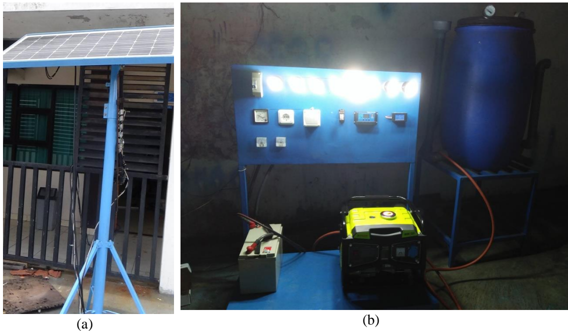
Figure 4. Research instrument (a) solar-PV, (b) Biogas power plant
