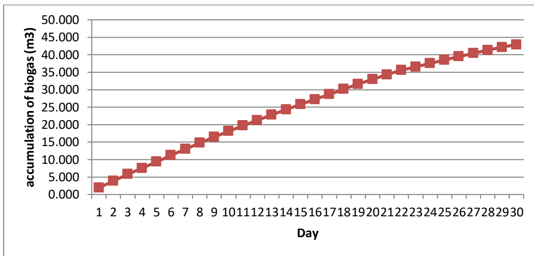
Figure 6. Accumulation of biogas production
