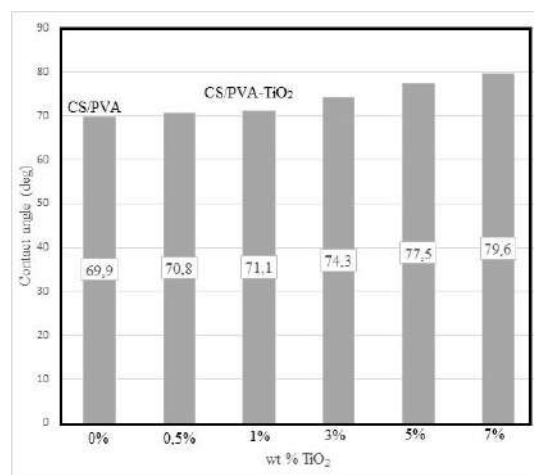
Fig. 8. The water contact angle of CS/PVA nanocomposite film vs CS/PVA- \text{TiO}_2 nanocomposite film
