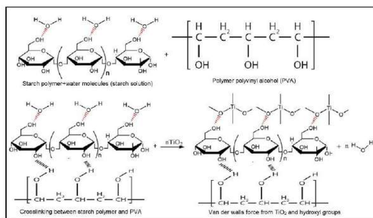
Fig. 5. Morphology surface and reaction between TiO 2 and polymer OH: a - surface photographs of CS/PVA without TiO 2 and with TiO 2 , b- hydroxyl groups adsorbed on nano-TiO 2 surface
