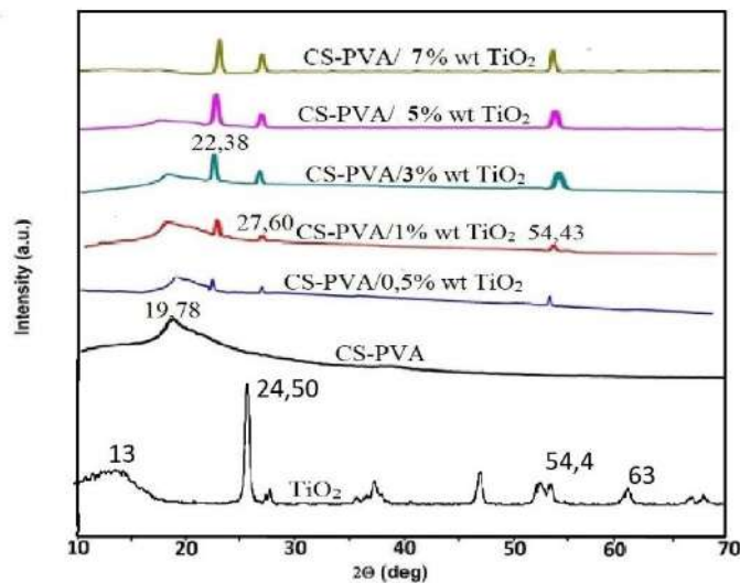
Fig. 4. XRD patterns for \text{TiO}_2 nanoparticle, CS/PVA, and CS/PVA- \text{TiO}_2 nanocomposite. Why is not represented a pure \text{TiO}_2 recorded spectrum?
