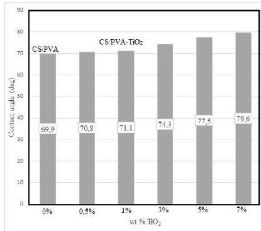
Fig. 8. The water contact angle of CS/PVA nanocomposite film vs CS/PVA-TiO 2 nanocomposite film
