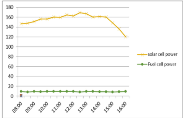
Figure 9. Charts hybrid power plant.
