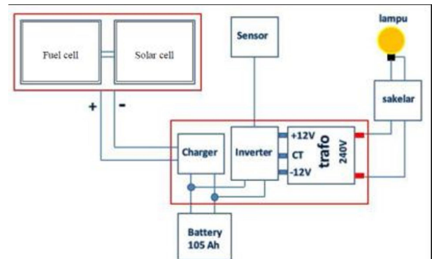
Figure 9. The hybrid power generation system
