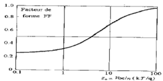
Figure 7. The form factor FF as a function zo
