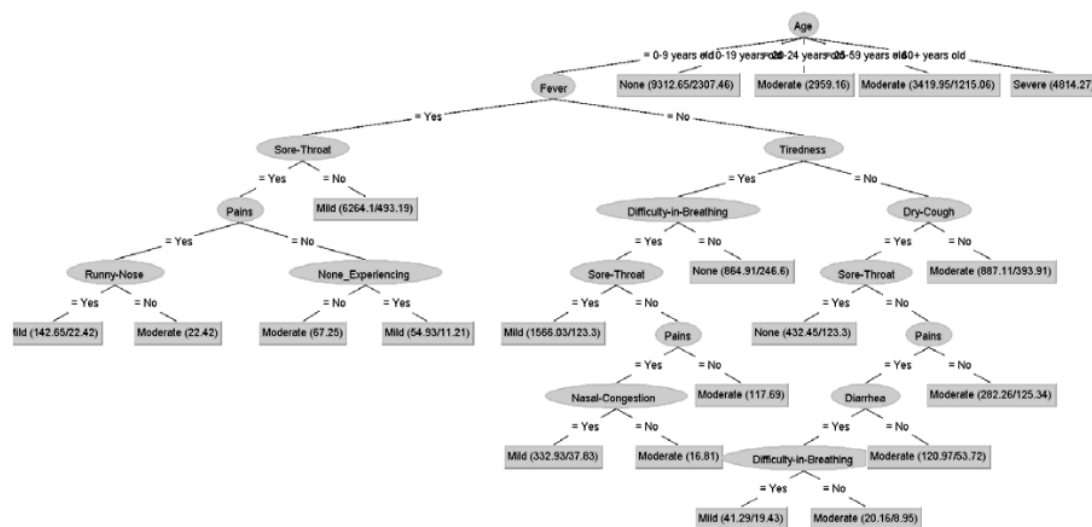
Fig. 2. Tree View of J48 using 10 fold cross-validation
