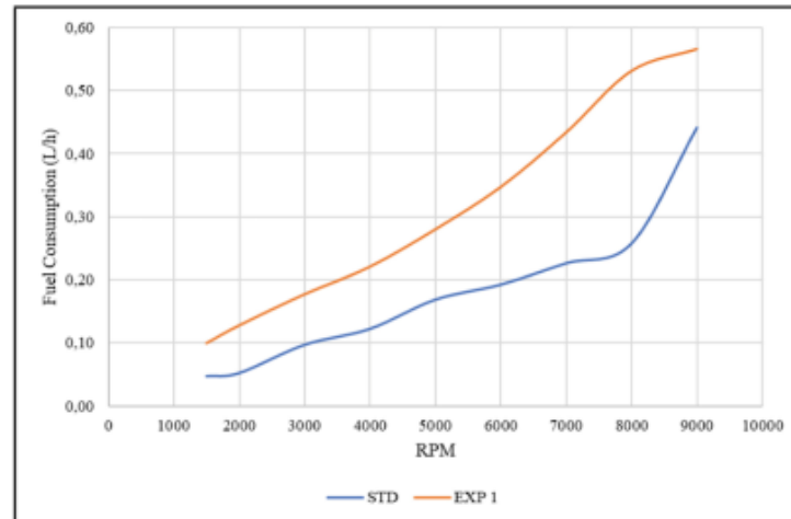
Fig. 3. Fuel Consumption Graph.
