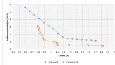
Figure 4 CO emission graph versus lambda.
