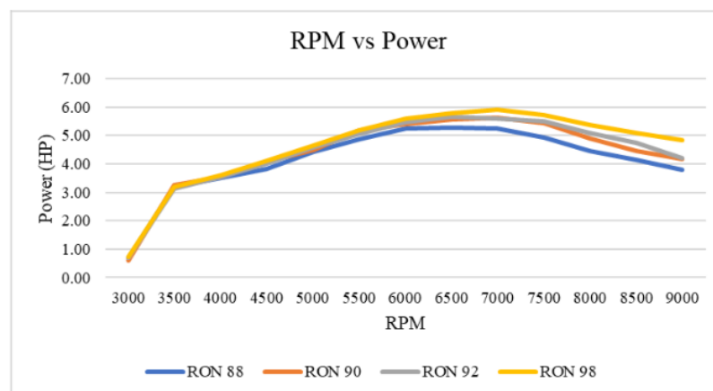
Figure 2. RPM test results with power.
