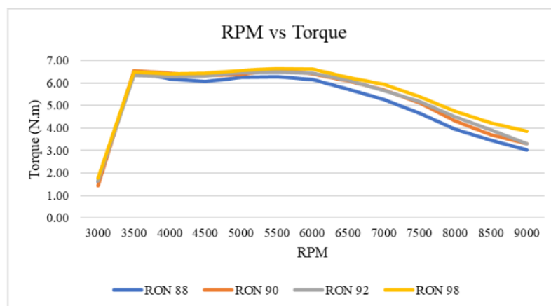
Figure 3. RPM test results with torque..
