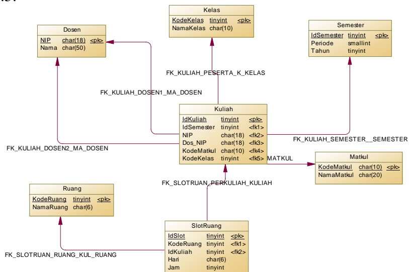
Gambar 6. PDM Reservasi Ruang
