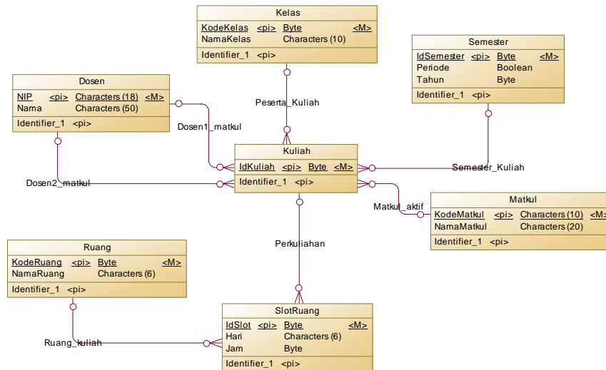
Gambar 5. CDM Reservasi Ruang
