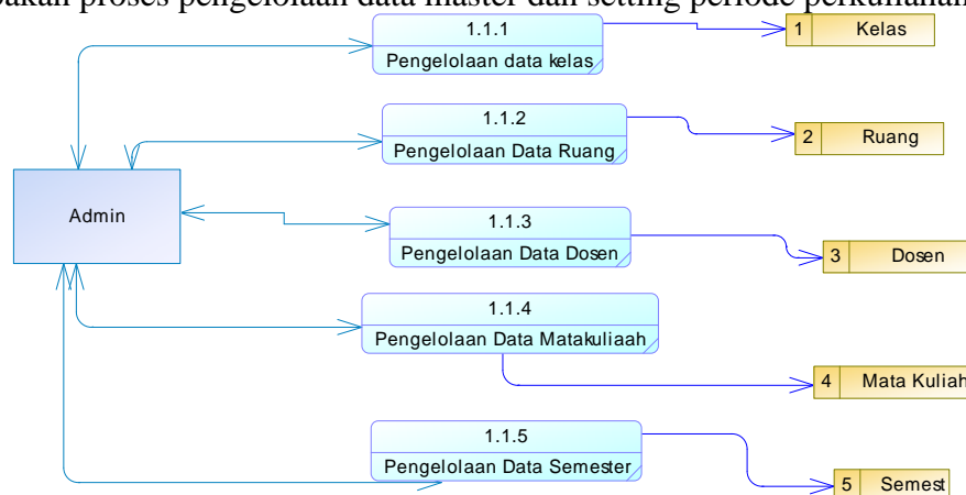
Gambar 4. DFD level 2 Mastering Data
