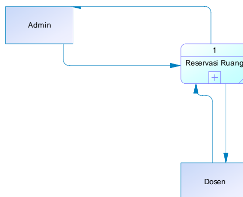
Gambar 2. DFD level 0
