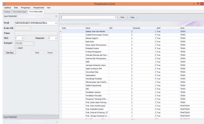
Gambar 9. Data Matakuliah
