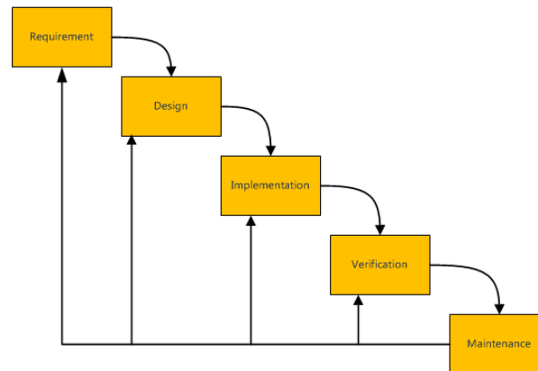
Gambar 1. Metode Waterfall
